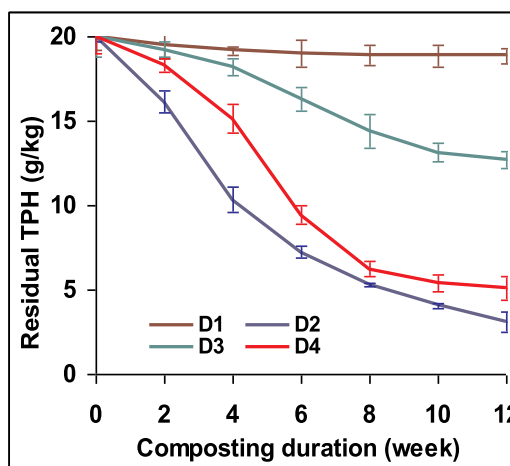
Fig. 4. Trend of TPHs degradation in the composting reactors over the process duration (D 1 : autoclaved PWS + autoclaved FC with no PDB inoculation as a control experiment; D 2 : autoclaved PWS + autoclaved FC + PDB inoculation; D 3 : autoclaved PWS + non-autoclaved FC; D 4 : autoclaved PWS + non-autoclaved FC + PDB inoculation).
