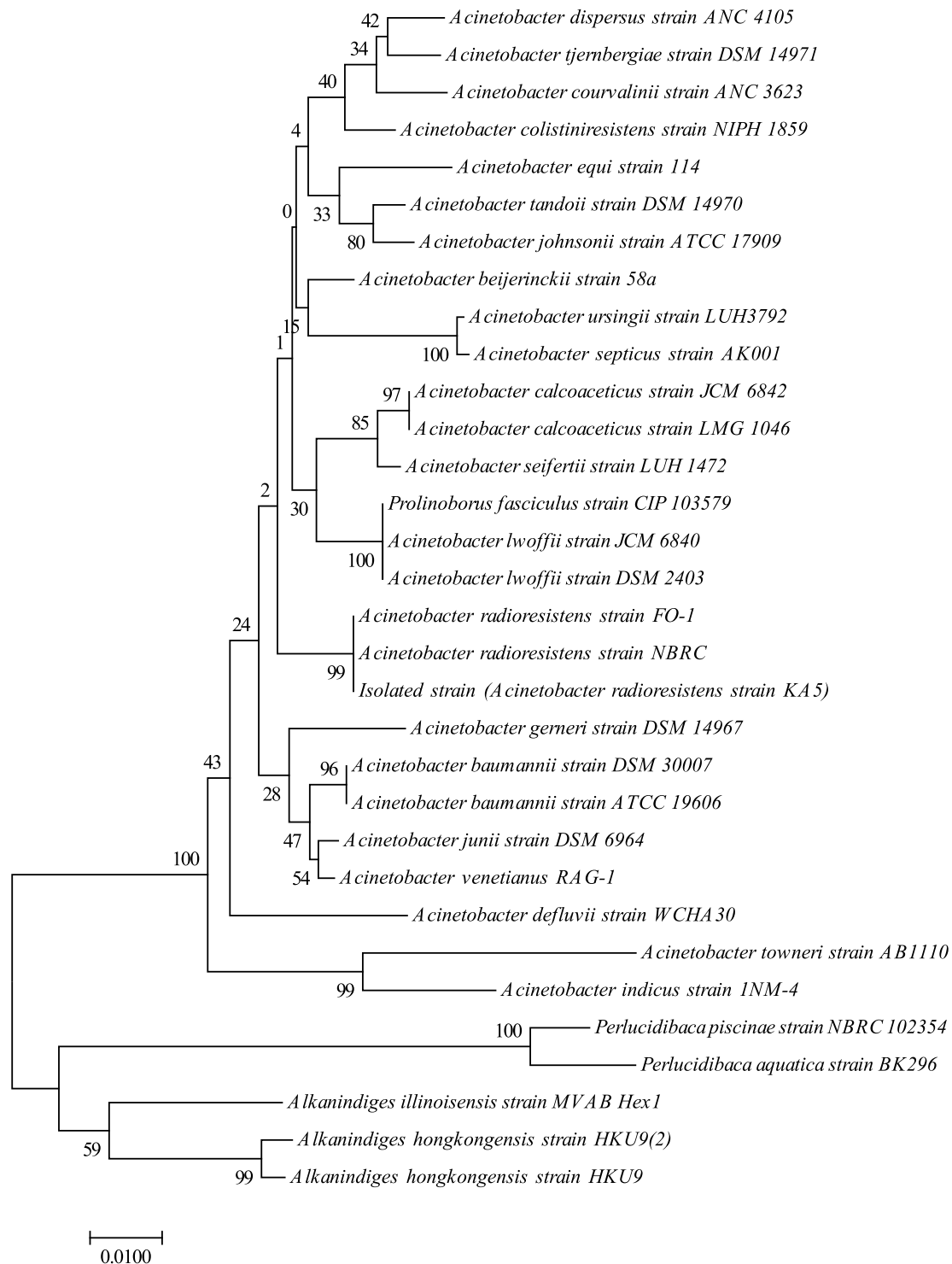
Fig. 1. Phylogenetic tree based on 16S rRNA gene sequences of Acinetobacter radioresistens strain KA5 isolated from the petroleum waste sludge.
