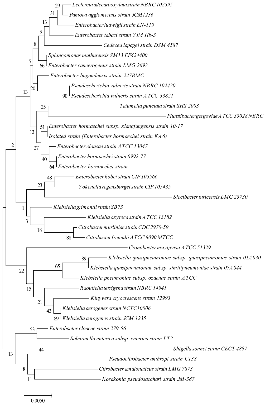
Fig. 2. Phylogenetic tree based on 16S rRNA gene sequences of Enterobacter hormaechei strain KA6 isolated from the petroleum waste sludge.
